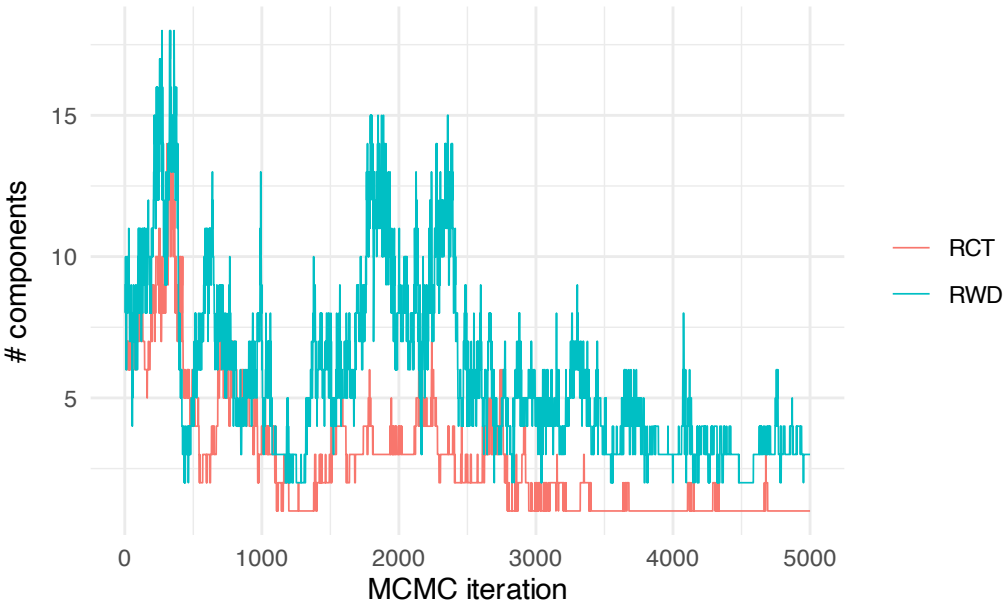
Occupied HDP components per source (pi > 0.01)
