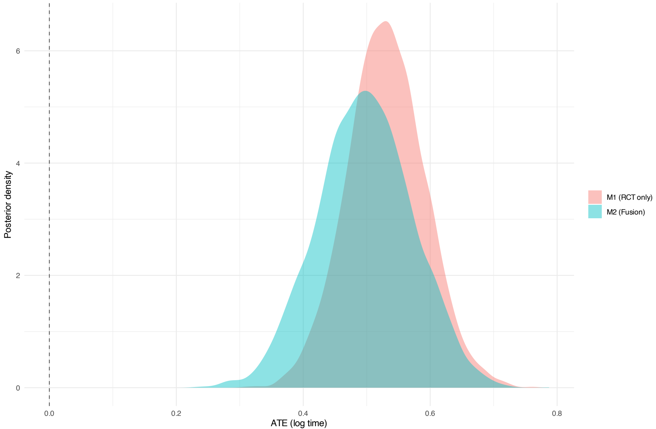
Average treatment effect (Bayesian bootstrap): M1 over F_RCT, M2 over combined cohort
